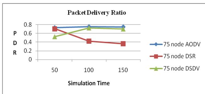
Fig 7 Comparison Graph between Packet Delivery Ratio vs Simulation time at 75 nodes
