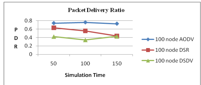
Fig 8 Comparison Graph between Packet Delivery Ratio vs Simulation time at 100 nodes
