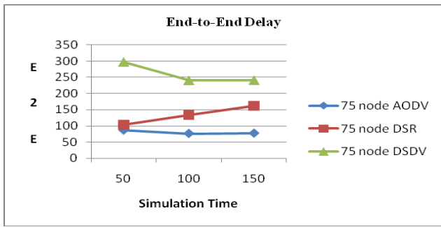
Fig 10 Comparison Graph between End-to-End Delay vs Simulation time at 75 nodes
