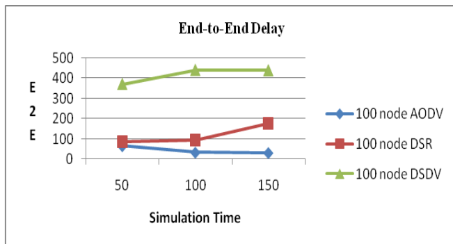
Fig 11 Comparison Graph between End-to-End Delay vs Simulation time at 100 nodes
