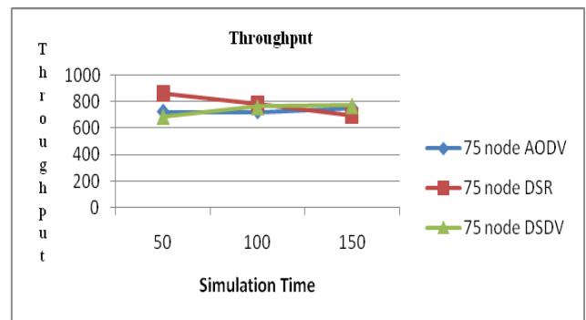
Fig 13 Comparison Graph between Throughput vs Simulation time at 75 nodes
