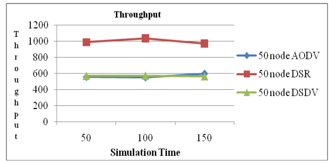
Fig 12 Comparison Graph between Throughput vs Simulation time at 50 nodes
