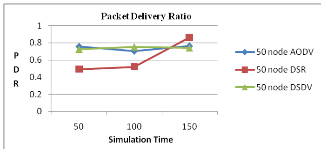
Fig 6 Comparison Graph between Packet Delivery Ratio vs Simulation time at 50 nodes
