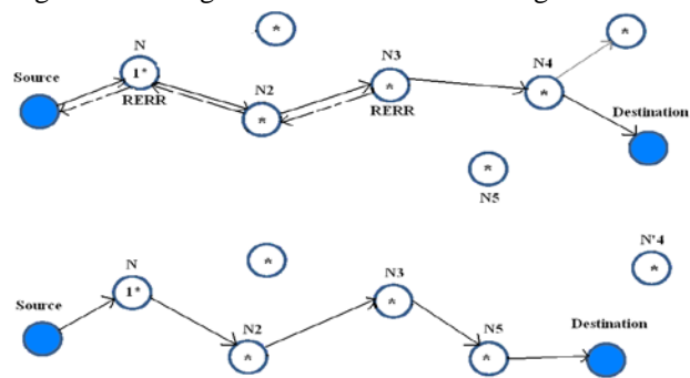
Fig 5 Route Request & Reply
